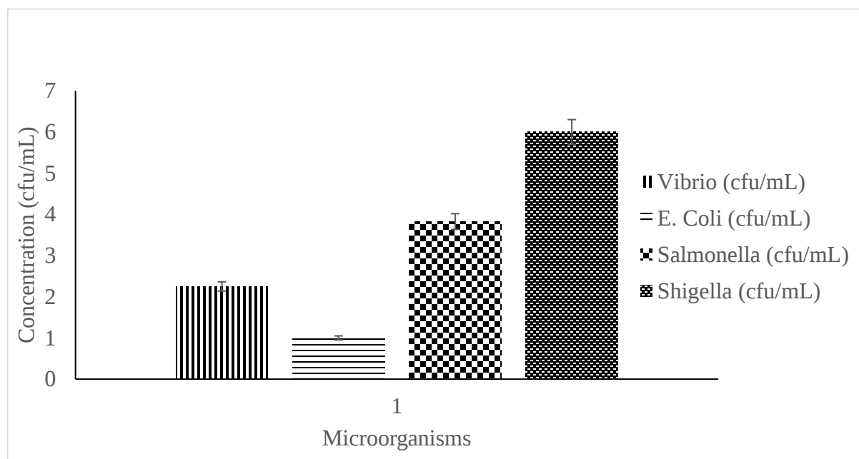
Fig. 6: Mean values of Microbial Activity for the Water Samples
