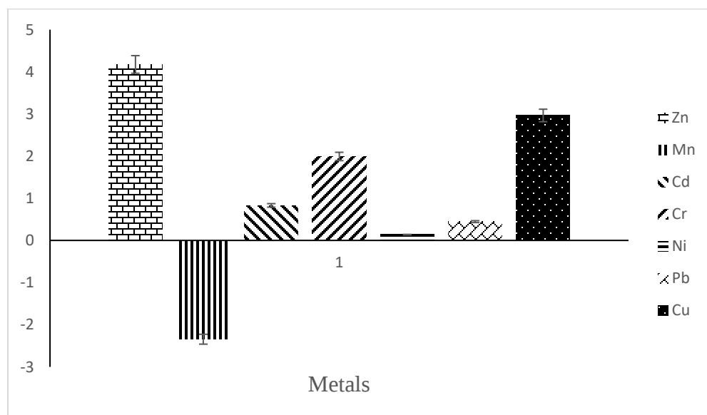
Fig.5: Mean and Standard Deviation of Geo-Accumulation Index for the Water Samples
